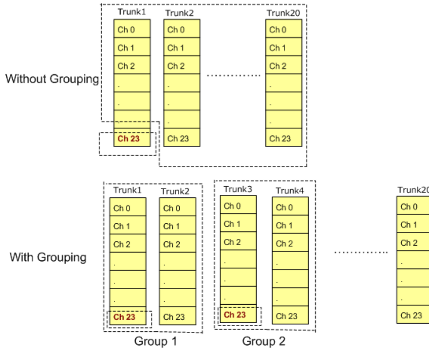
Figure: NFAS Grouping Illustration
