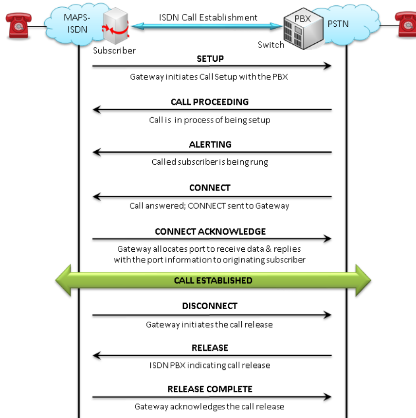
Figure: Typical ISDN Call Scenario
