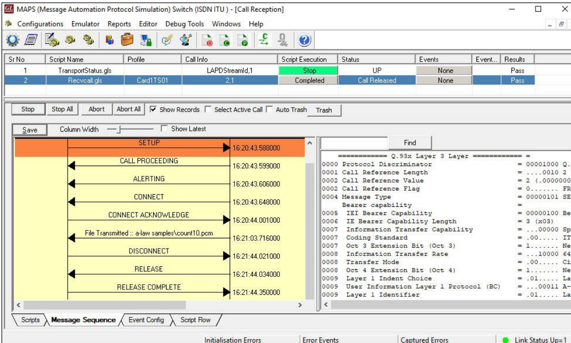
Figure: ISDN Signaling Call Reception
