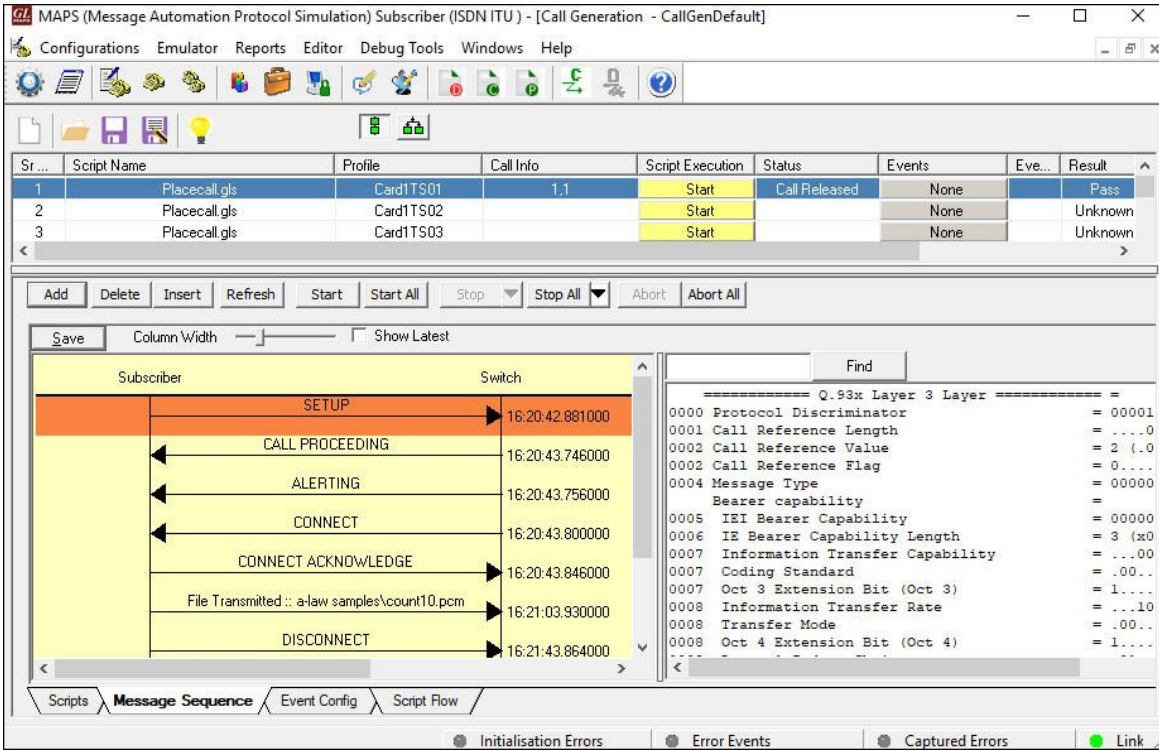
Figure: ISDN Signaling Call Generation
