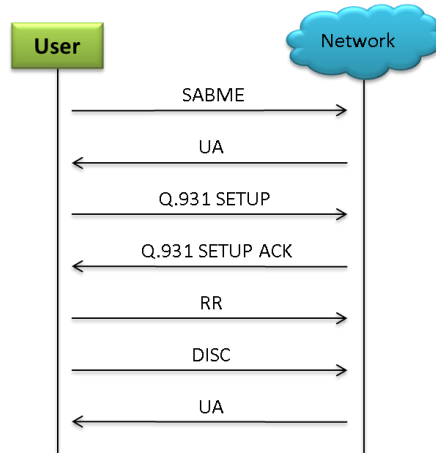
Figure: Typical LAPD Call Scenario
