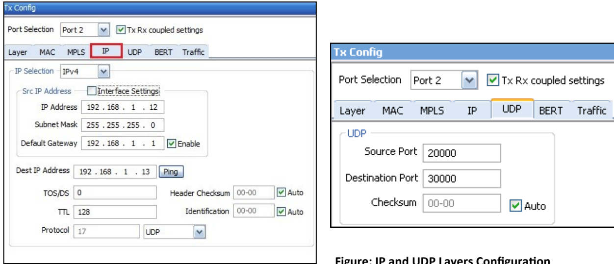
Figure: IP and UDP Layers Configuration
