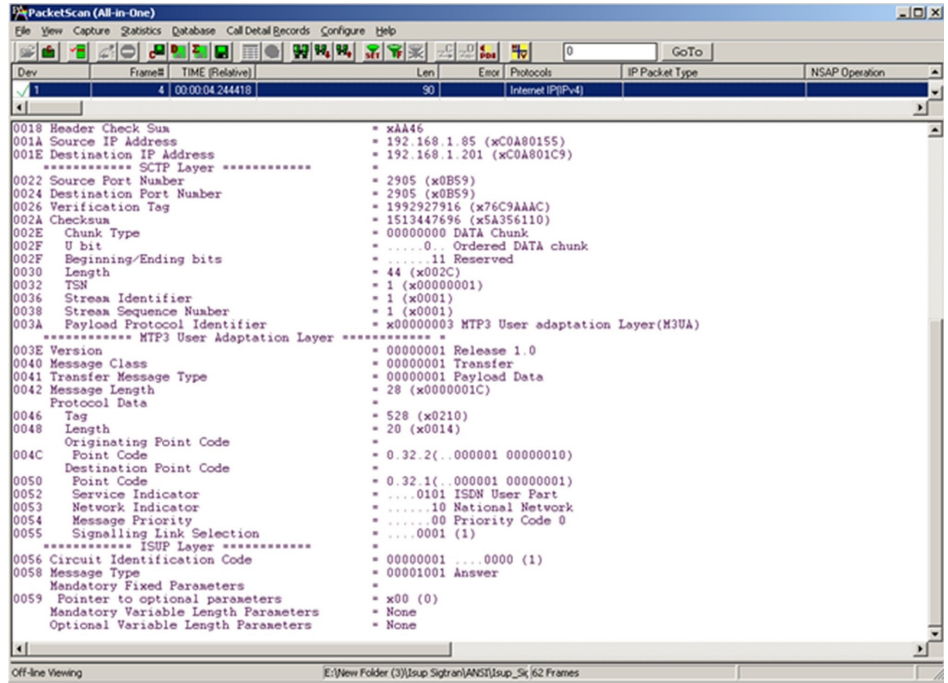
Figure: Detail View of SS7 SIGTRAN
